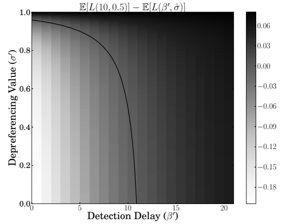
(b) Change in expected traffic loss
