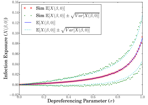
(b) Power-law website popularity
