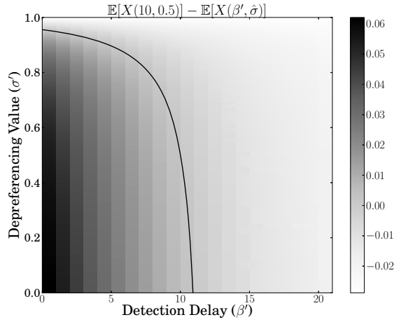
(a) Change in expected infection exposure
