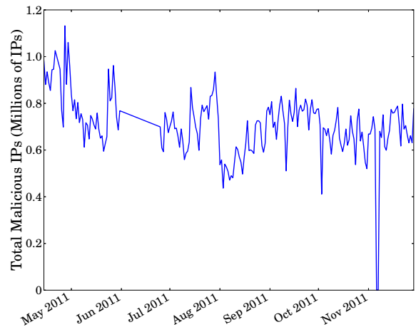
Figure 1: Variation in malicious IP addresses over time; from the Internet Storm Center ( http://isc.sans.org )
