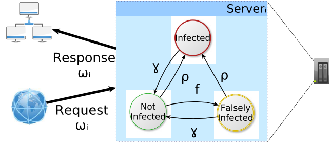
Figure 3: Model of website infections and client exposure.
