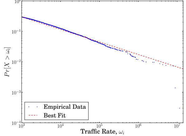
Figure 4: Empirically observed website traffic follows a power-law distribution with \alpha = -1.4 .
